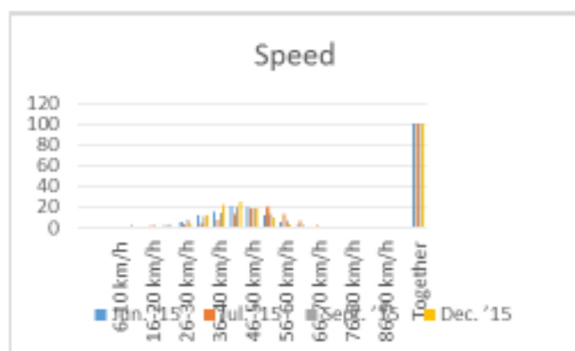
Graph I: Speed monitoring
